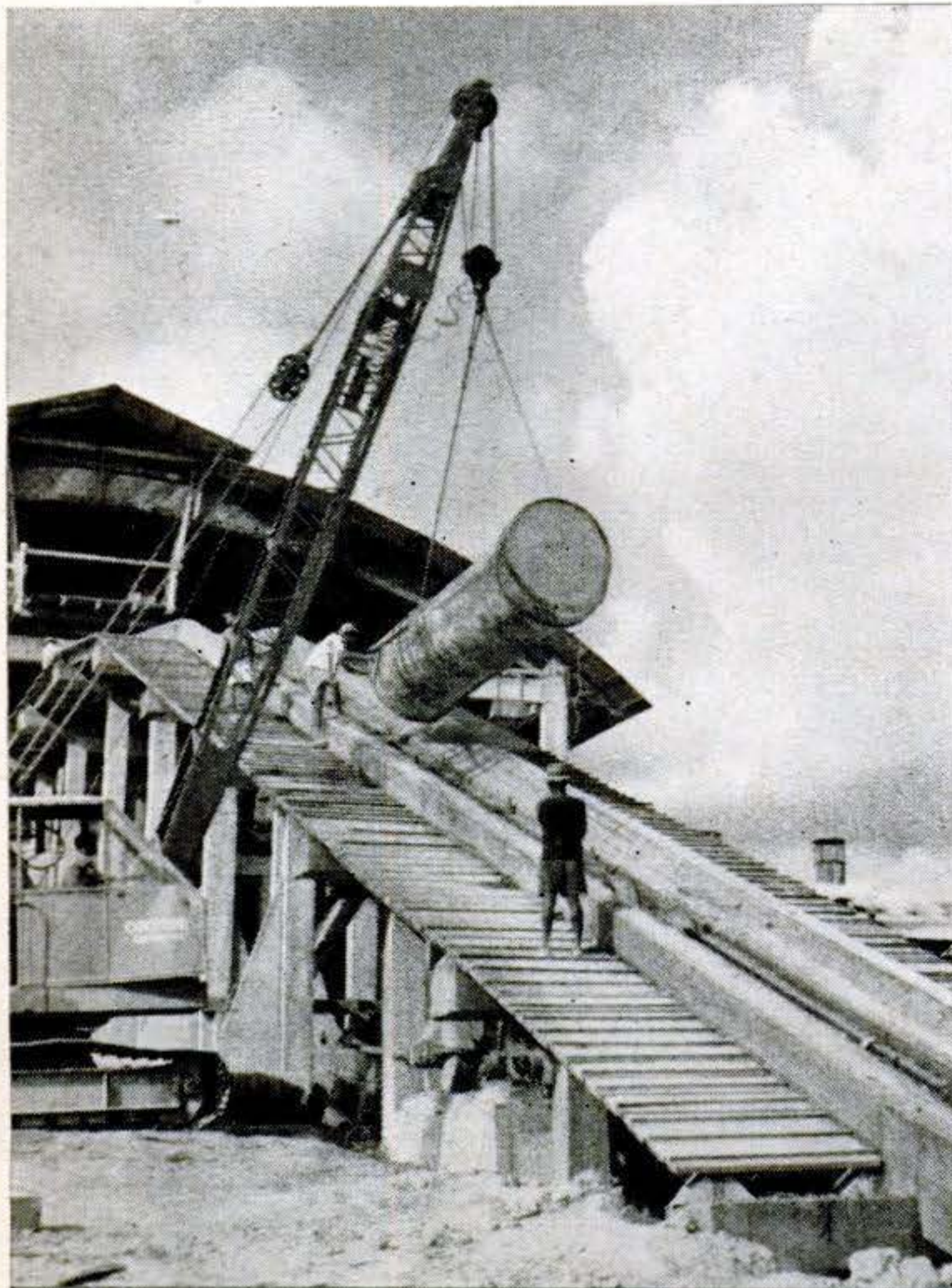
AFTER BEING CUT IN TWO SECTIONS , one part of the log is swung over the ramp onto a conveyor belt that takes it into the sawmill. Natives above guide log as a crane lowers it.
